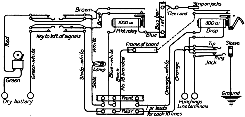
COM. BAT. LINE CIRCUIT - VIS. SIGS.
